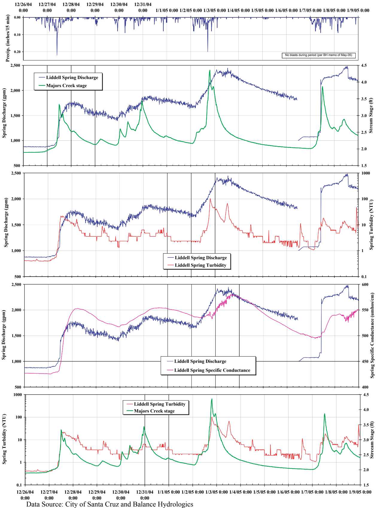
Storm Hydrograph Comparison, December 2004 - January 2005
